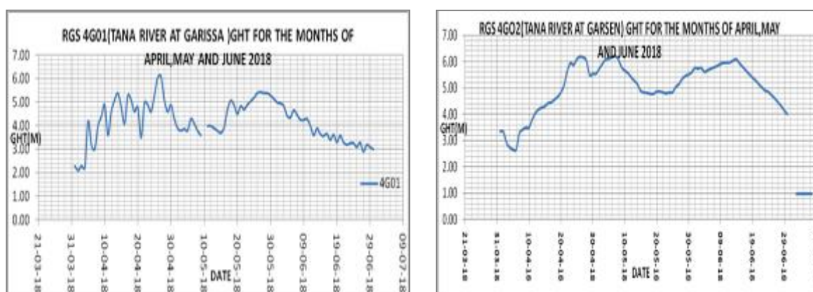
Figure 3.8: Water level hydrograph at Tana river 4G01 and 4G02
