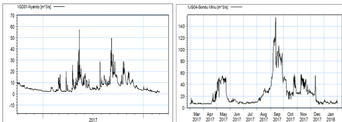
Figure 3.6: Streamflow hydrographs for Nyando 1GD03 and Sondu river 1JG04
